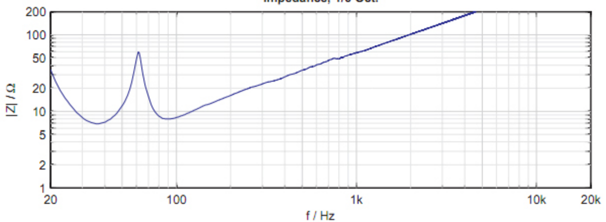
Impedance, 1/6 Oct.
